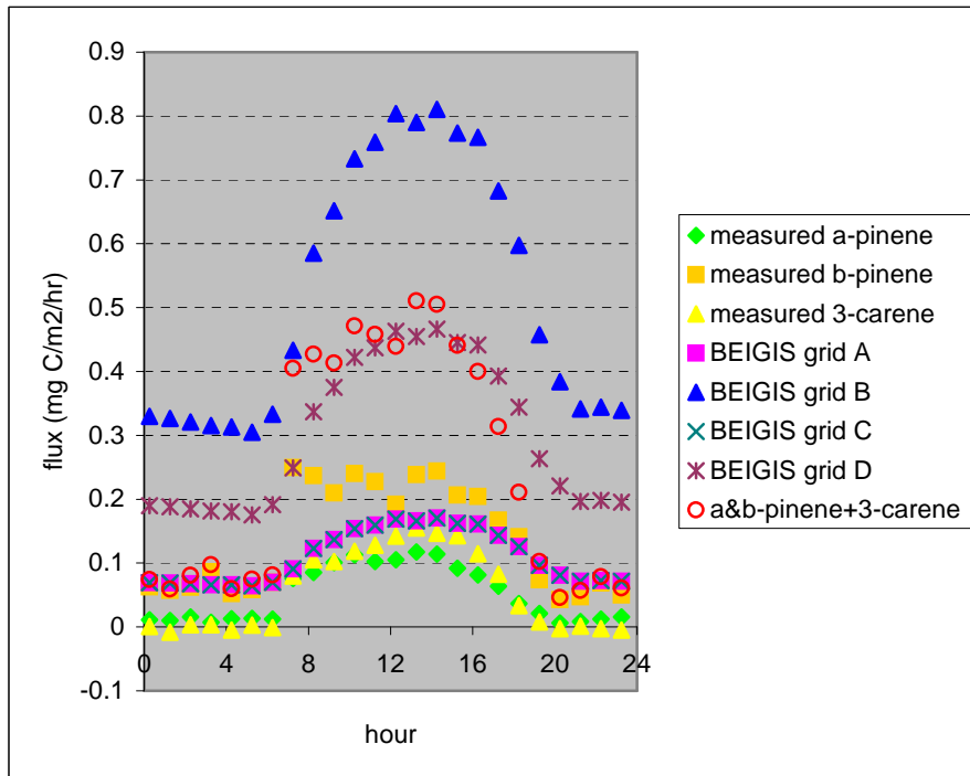
Figure B-4. Monoterpene fluxes modeled with default BEIGIS inputs, vs. measured monoterpene fluxes.
