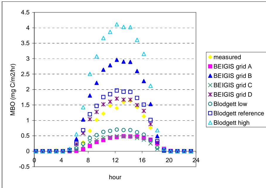
Figure B-3. MBO fluxes modeled with default BEIGIS vs. on-site Blodgett inputs, compared to measured fluxes.
