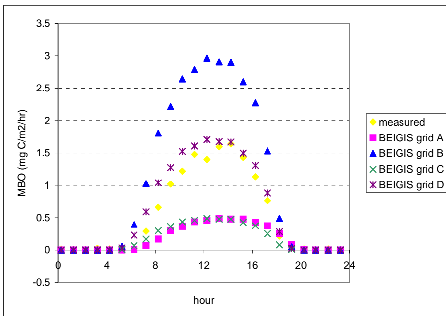
Figure B-2. Measured vs. modeled MBO fluxes.
