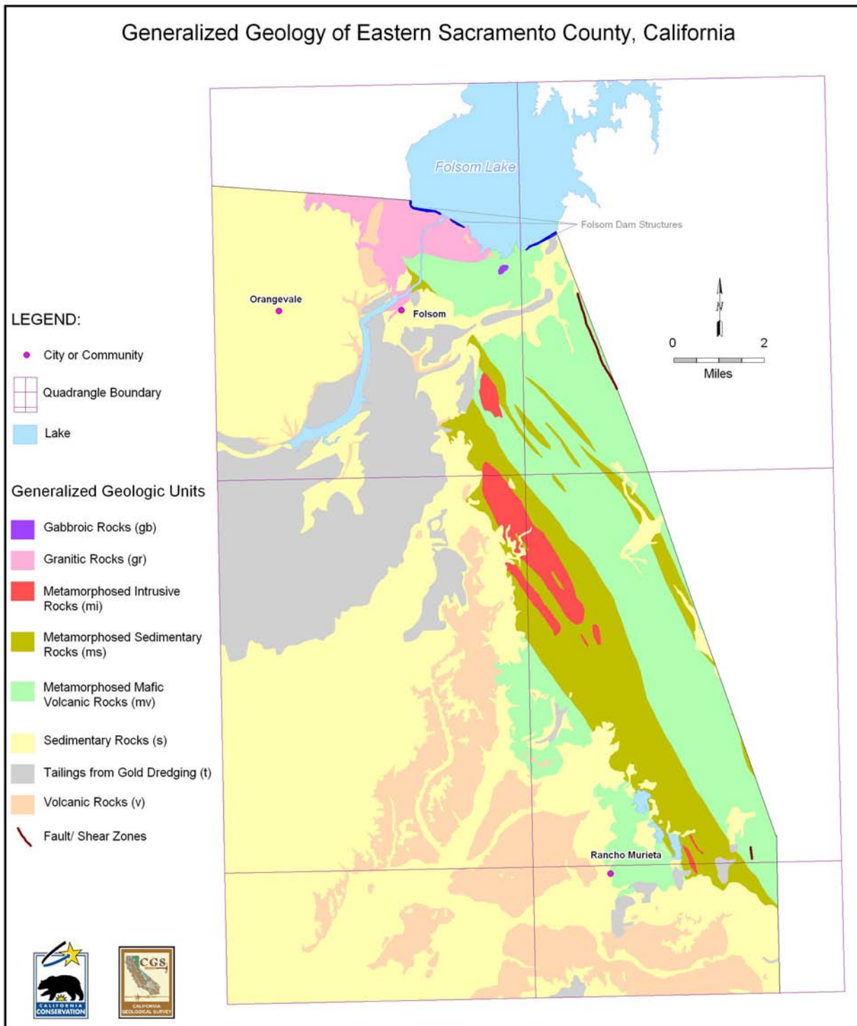
Figure 2. Generalized Geologic Map of Eastern Sacramento County.
